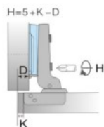
Hinge cup types
