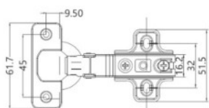
Hinge cup types
